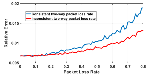
Fig. 13. Relative error change with packet loss rate (fix the packet loss rate for one of the receivers as 0.1).
