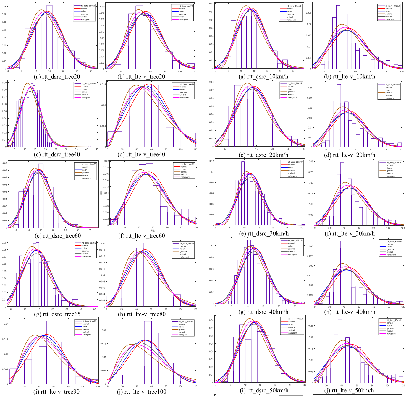
Fig. 18. PDF of the V2I communication delay in the environment with shelters (trees in this experiment).
