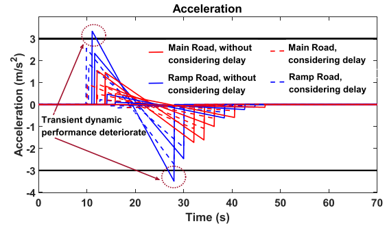
Fig. 7. Control inputs (acceleration) of the vehicles, Case 1.
