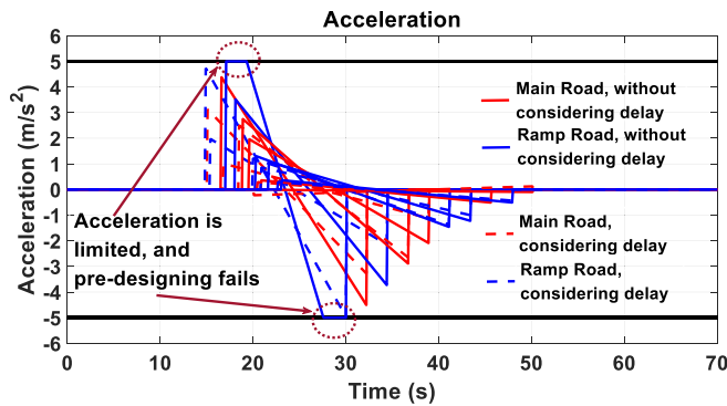
Fig. 10. Control inputs (acceleration) of the vehicles, case 2.
